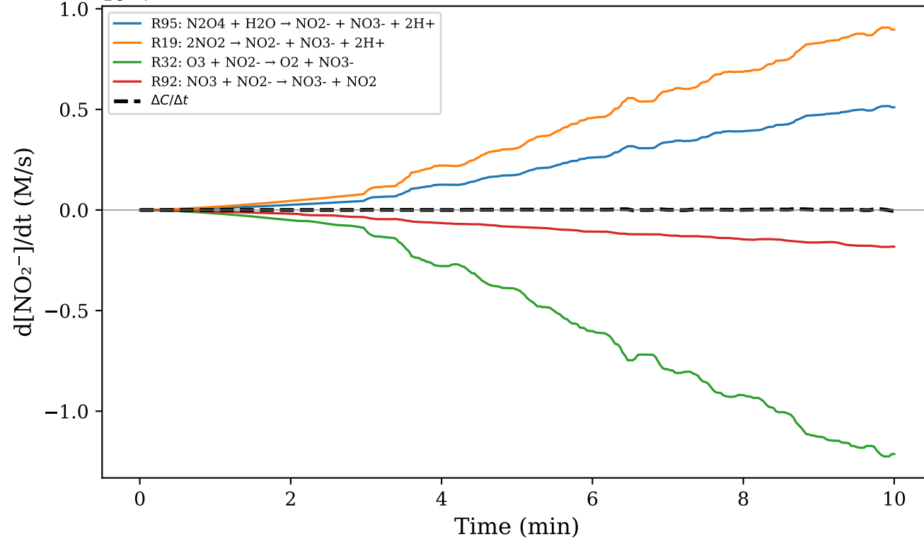
(c) \text{NO}_2^-
